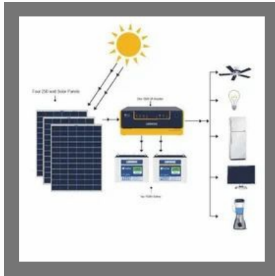
Solar Rooftop Off Grid System
